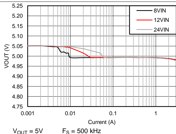
Figure 9. V_{OUT} Regulation
