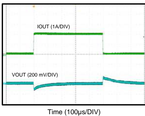
Figure 81. Output Voltage Regulation
