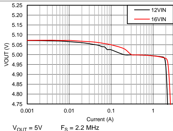
Figure 11. V_{OUT} Regulation
