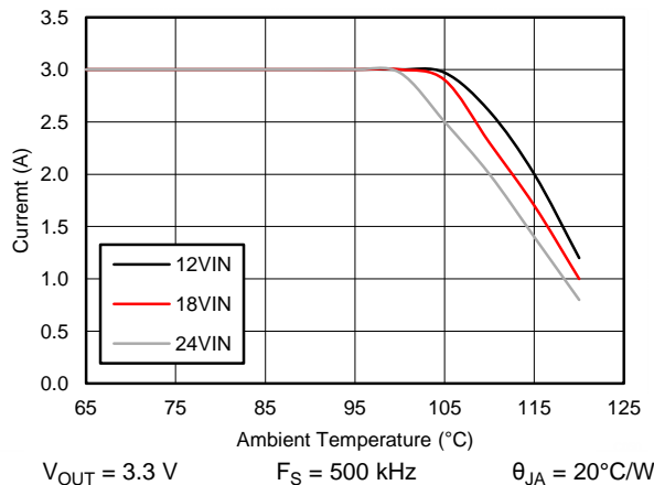
Figure 66. Derating Curve
