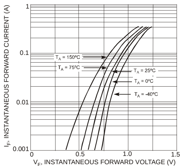
Fig. 2 Forward Characteristics
