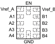
图 6-3. RUT Package, 12-Pin UQFN (Transparent Top View)
