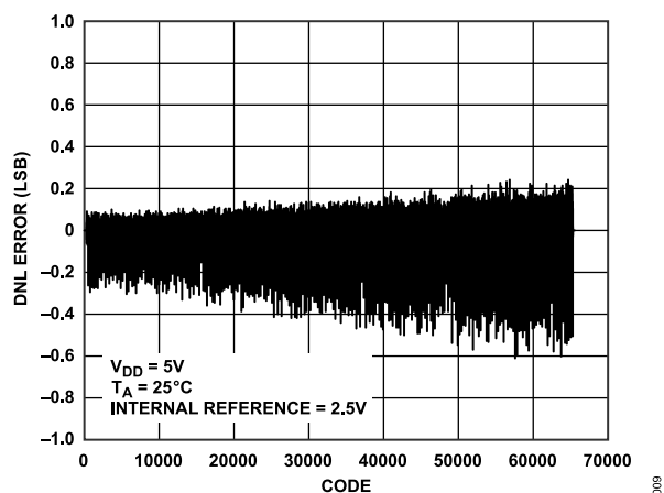
Figure 11. AD5676R DNL Error vs. Code
