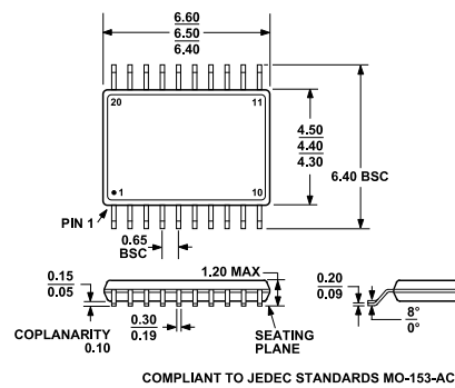
Figure 73. 20-Lead Thin Shrink Small Outline Package [TSSOP] (RU-20) Dimensions shown in millimeters
