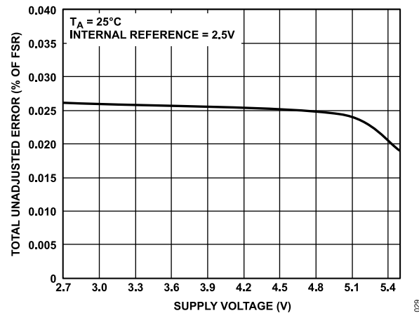
Figure 24. AD5676R TUE vs. Supply Voltage
