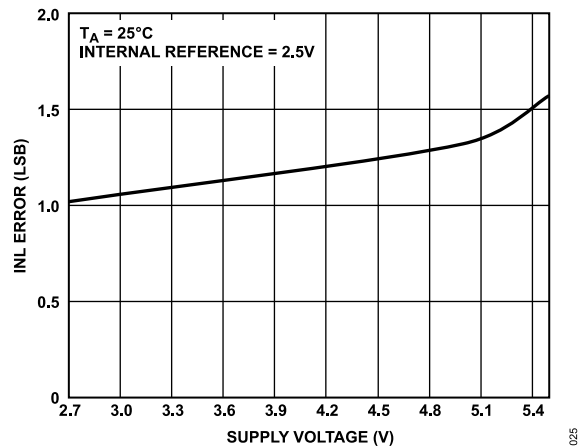
Figure 21. AD5676R INL Error vs. Supply Voltage
