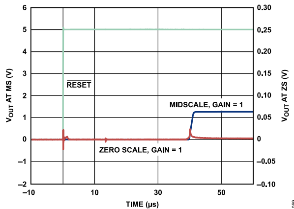
Figure 52. Hardware Reset
