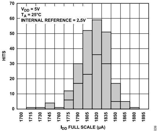
Figure 33. Supply Current ( I_{DD} ) Histogram with Internal Reference
