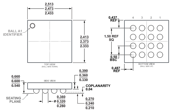
Figure 75. 16-Ball Wafer Level Chip Scale Package [WLCSP] (CB-16-24) Dimensions shown in millimeters
