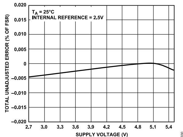
Figure 25. AD5672R TUE vs. Supply Voltage
