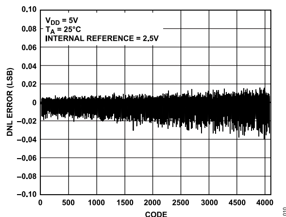
Figure 12. AD5672R DNL Error vs. Code
