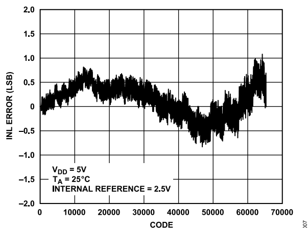
Figure 9. AD5676R INL Error vs. Code
