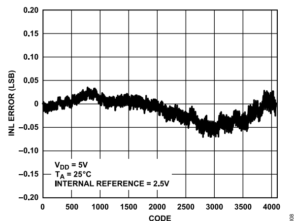
Figure 10. AD5672R INL Error vs. Code
