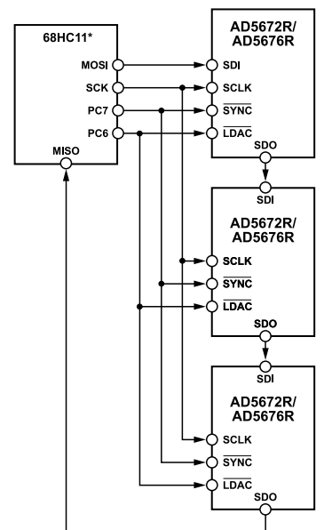
Figure 62. Daisy-Chaining the AD5672R/AD5676R
