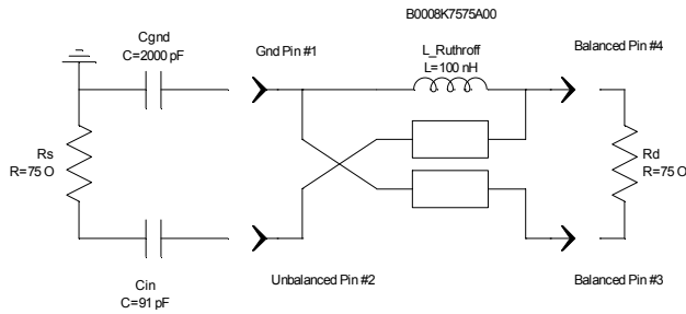
Figure 3 The Balun with an external inductor in a Ruthroff implementation with an external 100 nH inductor and DC block to enhance insertion and return loss. Data is compared to the basic Guanella configuration (dashed lines). Other capacitor and inductor values can be used with different results.
