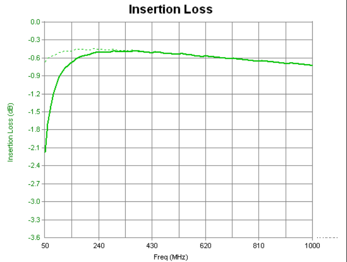
Figure 2 The Balun with an external inductor in a Ruthroff implementation with an external 100 nH inductor. Data is compared to the basic Guanella configuration (dashed lines). Other inductor values can be used with different results.
