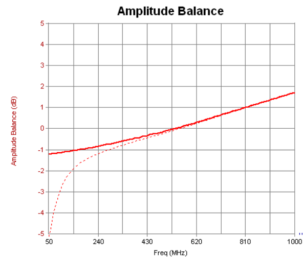
Figure 2 The Balun with an external inductor in a Ruthroff implementation with an external 100 nH inductor. Data is compared to the basic Guanella configuration (dashed lines). Other inductor values can be used with different results.
