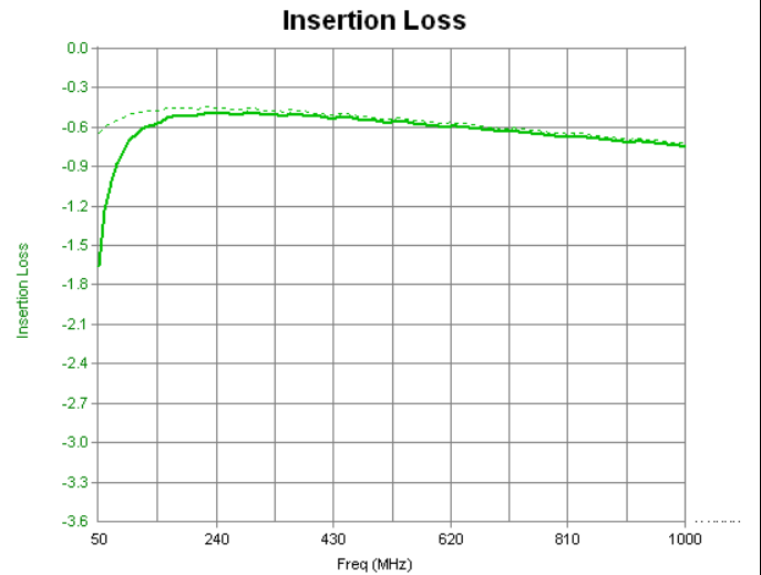
Figure 3 The Balun with an external inductor in a Ruthroff implementation with an external 100 nH inductor and DC block to enhance insertion and return loss. Data is compared to the basic Guanella configuration (dashed lines). Other capacitor and inductor values can be used with different results.
