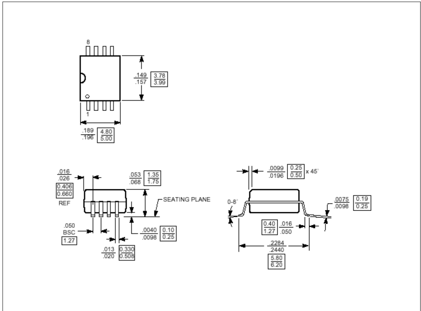
Figure 7. 8-Pin SOIC
