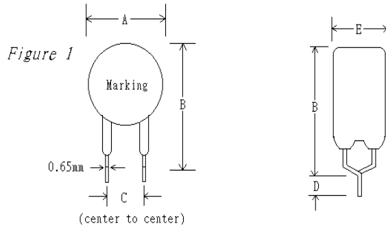
Figure 1 Lead Size: 22AWG Φ 0.65 mm Diameter
