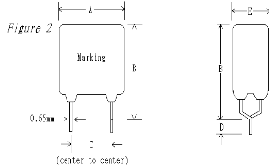
Figure 2 Lead Size: 22AWG Φ 0.65 mm Diameter
