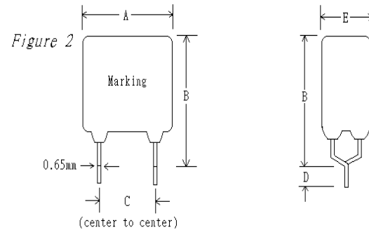
Figure 2 Lead Size: 22AWG Φ 0.65 mm Diameter
