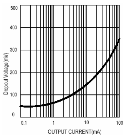
Fig 6. Dropout Voltage
