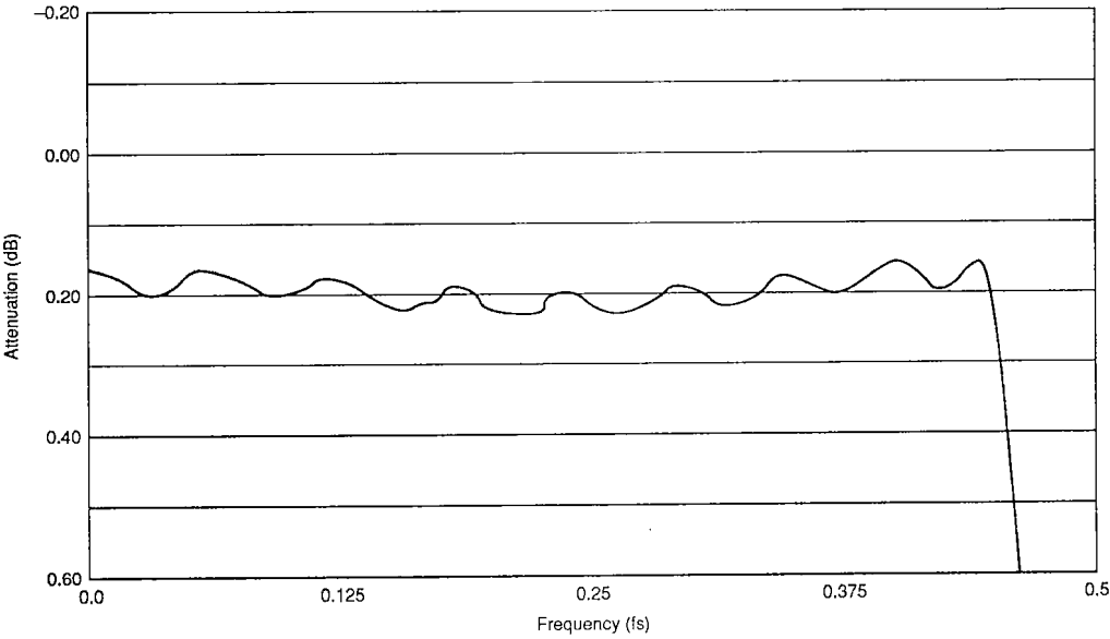
4fs filter passband characteristic (Deemphasis OFF)
