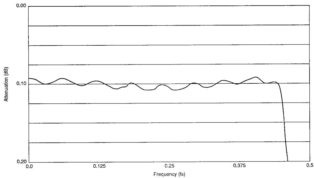
8fs filter band-transition characteristic (Deemphasis OFF)
