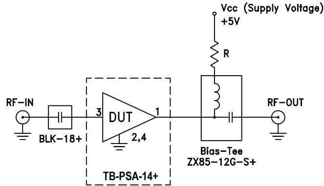
Fig 1. Block Diagram of Test Circuit used for characterization. (DUT soldered on Mini-Circuits Characterization test board TB-PSA-14+) Gain, Return loss, Output power at 1dB compression (P1 dB) , output IP3 (OIP3) and noise figure measured using Agilent’s N5242A PNA-X microwave network analyzer. (R=16.5Ω)
