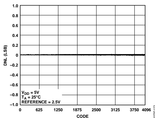
Figure 11. AD5684 DNL
