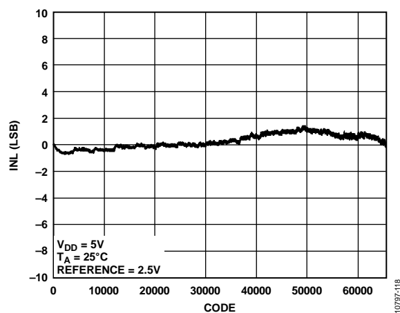
Figure 8. AD5686 INL
