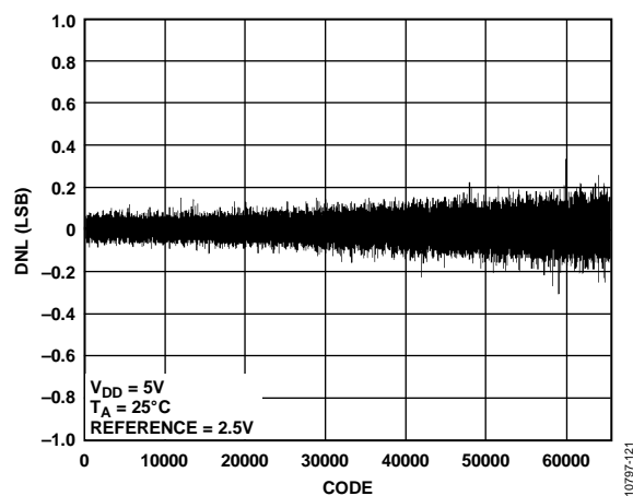
Figure 10. AD5686 DNL
