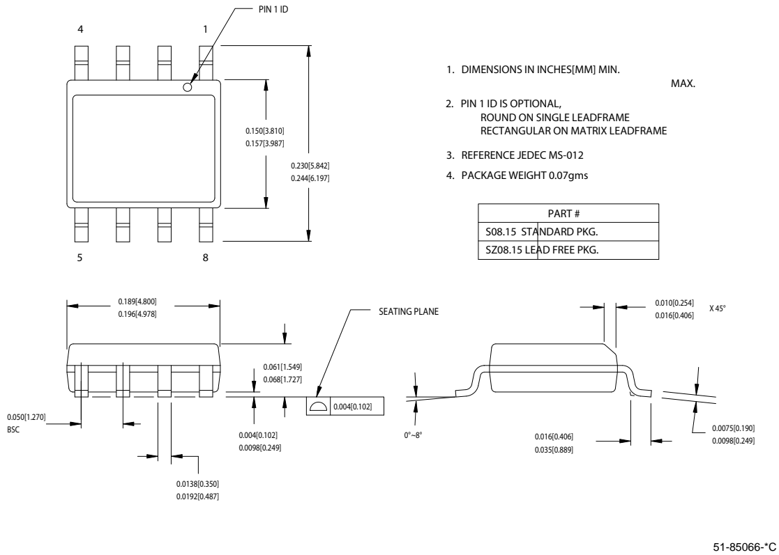
Figure 13. 8-Pin (150-Mil) SOIC (51-85066)
