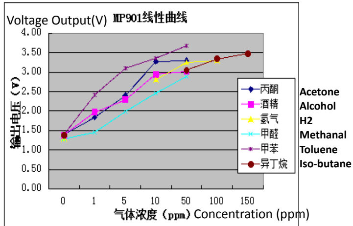
Fig6. Linearity curve
