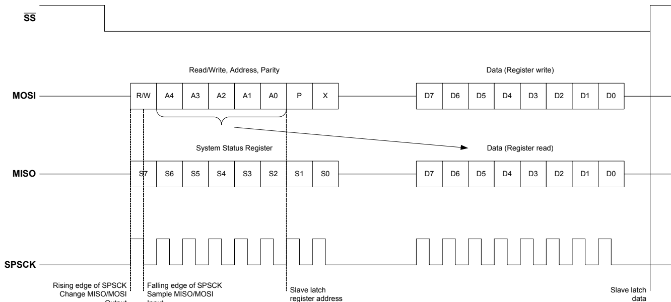
Figure 31. SPI Protocol
