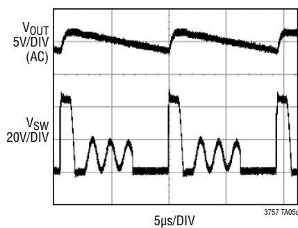
Switching Waveforms
