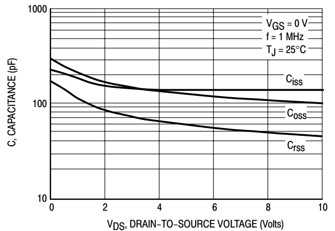
Figure 8. Capacitance
