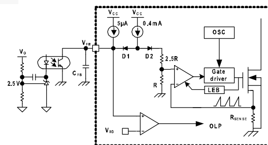
Figure 16. Pulse-Width-Modulation Circuit
