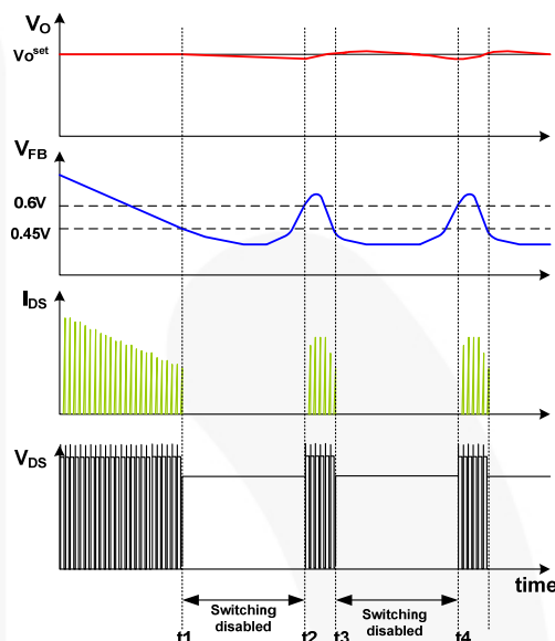
Figure 22. Burst-Mode Operation
