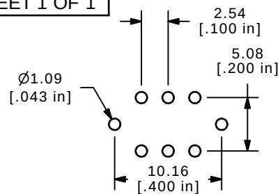
P.C. MOUNTING
