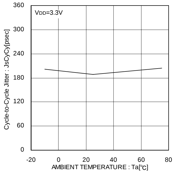
Figure 42. CLKOUT \pm 0.75\% Modulation Cycle-to-Cycle Jitter
