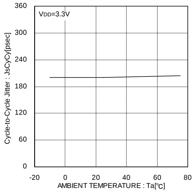
Figure 38. CLKOUT \pm 0.25\% Modulation Cycle-to-Cycle Jitter
