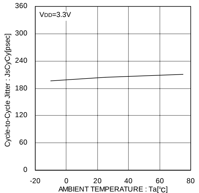
Figure 40. CLKOUT \pm 0.50\% Modulation Cycle-to-Cycle Jitter
