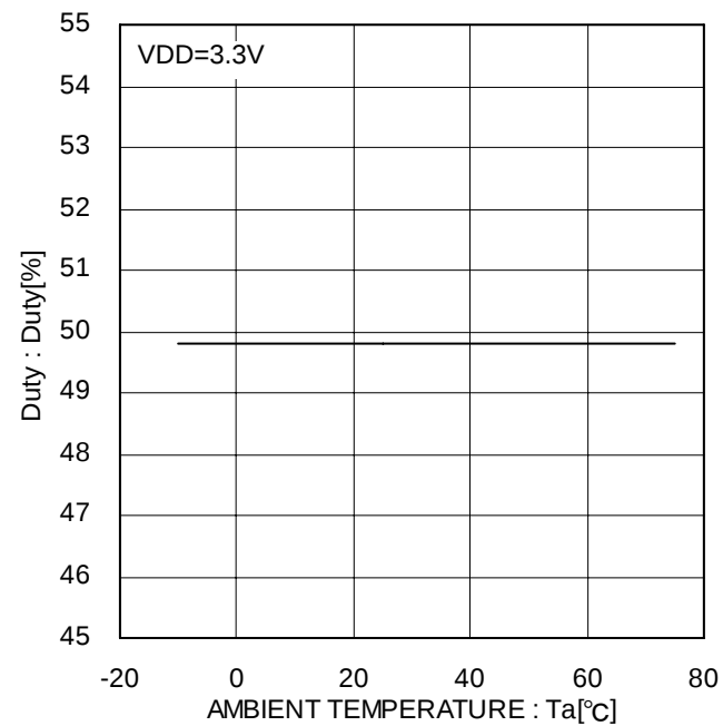
Figure 20. CLKOUT Duty
