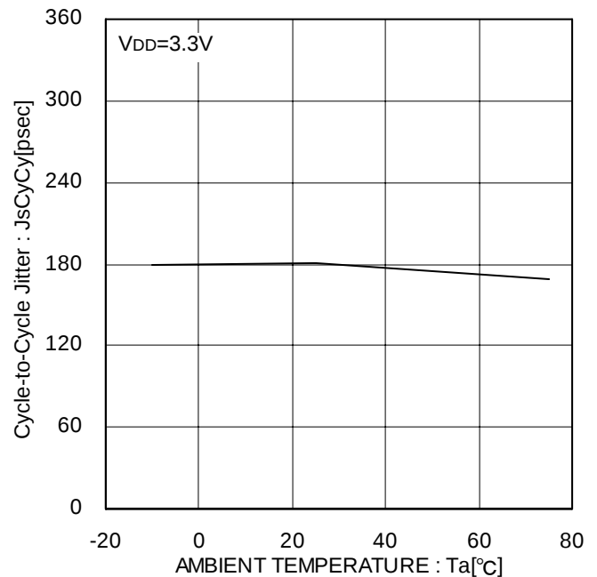
Figure 44. CLKOUT \pm 1.00\% Modulation Cycle-to-Cycle Jitter
