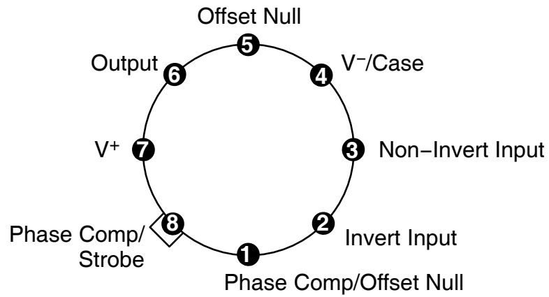
Pin Connection Diagram (Top View)
