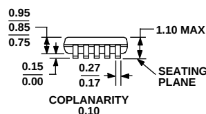
Figure 21. 10-Lead Mini Small Outline Package [MSOP] (RM-10)
