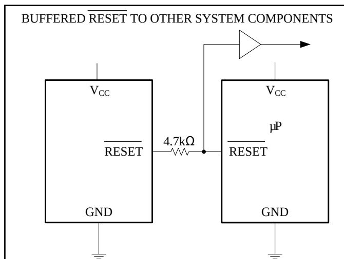
Figure 11. Bidirectional Reset I/O
