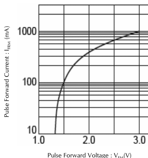
Pulse Forward Voltage vs. Pulse Forward Current
