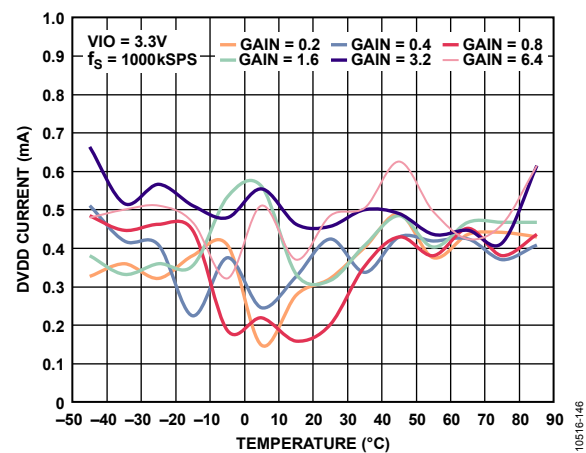
Figure 42. DVDD Current vs. Temperature
