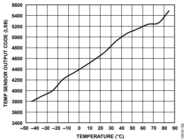
Figure 49. Temperature Sensor Output Code vs. Temperature
