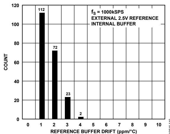
Figure 17. Reference Buffer Drift, External Reference
