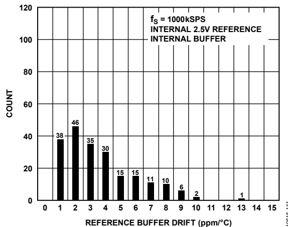
Figure 18. Reference Buffer Drift, Internal Reference
