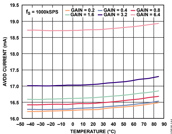
Figure 41. AVDD Current vs. Temperature
