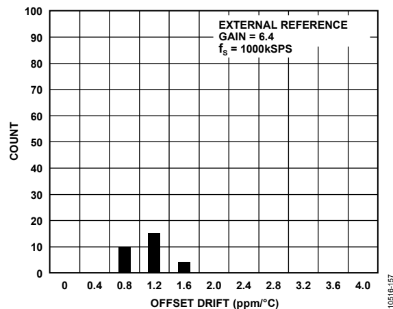
Figure 16. Offset Drift, PGIA Gain = 6.4
