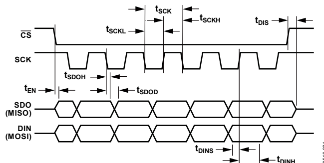
Figure 69. Serial Timing
