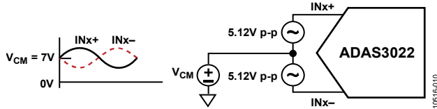
Figure 58. Differential, Antiphase Inputs with a Nonzero Common Mode
