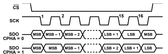
Figure 70. CPHA Details
