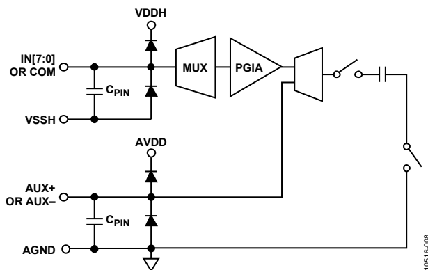
Figure 56. Equivalent Analog Input Circuit
