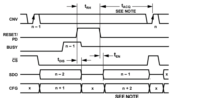
NOTES 1. WHEN THE PART IS RELEASED FROM RESET, t_{ACQ} MUST BE MET FOR CONVERSION n IF USING THE DEFAULT CFG SETTING FOR CHANNEL IN0. WHEN THE PART IS RELEASED FROM POWER-DOWN, t_{ACQ} IS NOT REQUIRED, AND THE FIRST TWO CONVERSIONS, n AND n + 1 , ARE UNDEFINED.
