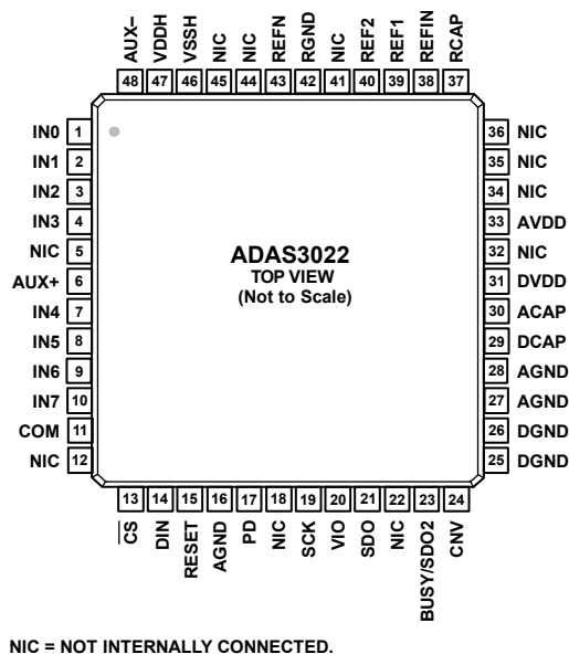
Figure 6. LQFP Pin Configuration
