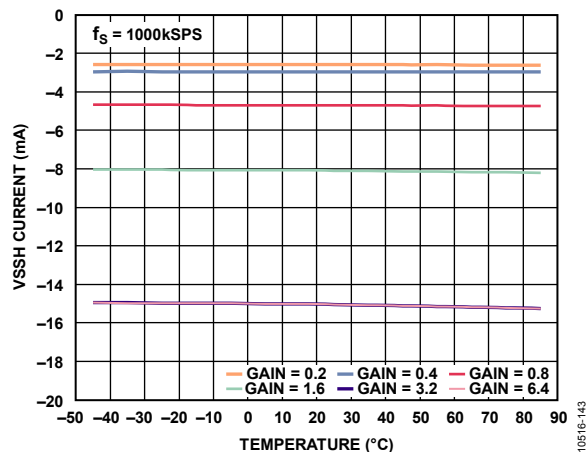
Figure 40. VSSH Current vs. Temperature
