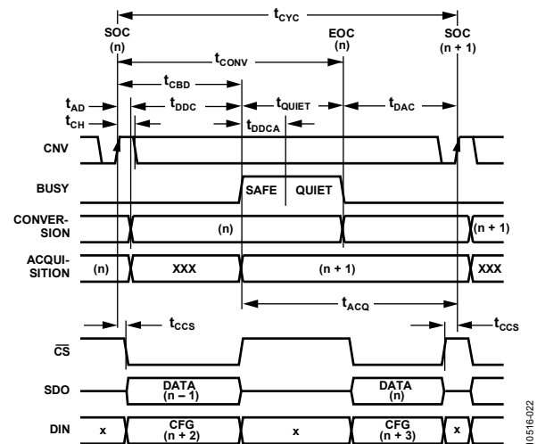
Figure 67. Basic Conversion Timing
