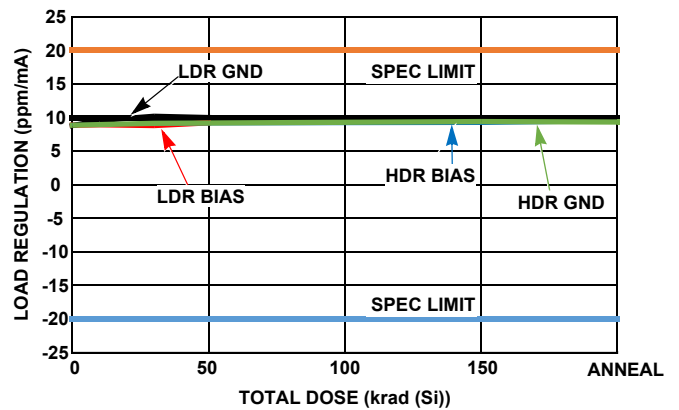
FIGURE 8. LOAD REGULATION (SOURCING) SHIFT
