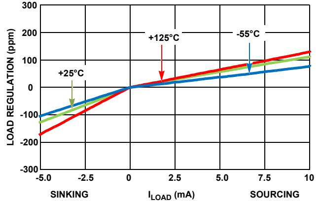
FIGURE 14. LOAD REGULATION vs V_{OUT} (PPM) OVER TEMPERATURE
