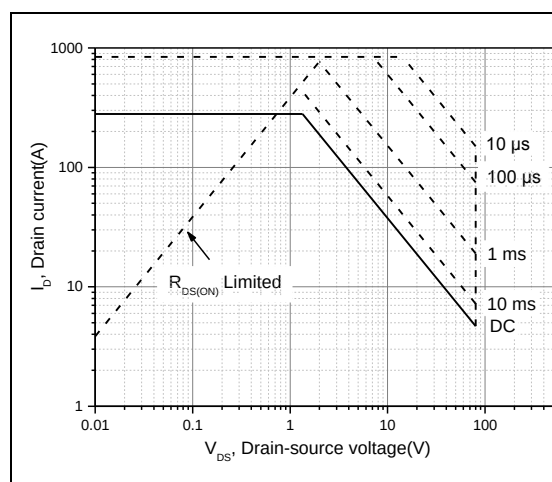
Figure 9, Safe operation area T_C = 25^\circ\text{C}
