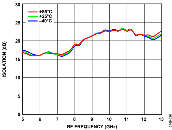
Figure 36. RF to IF Isolation vs. RF Frequency at Various Temperatures
