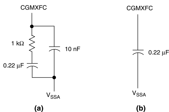
Figure 6-10. PLL Filter
