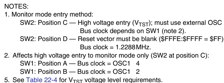
Figure 8-1. Monitor Mode Circuit
