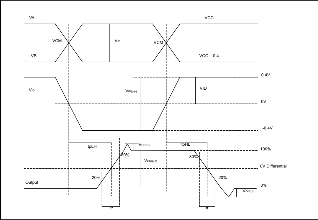
Figure 12. Propagation delays
