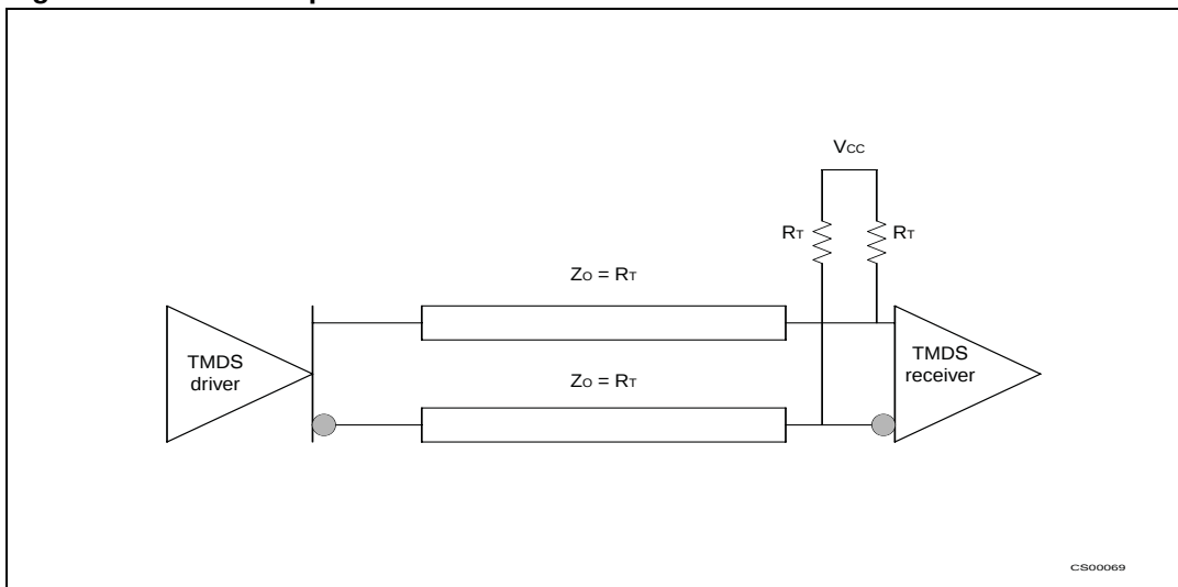
Figure 8. TMD5 output driver
