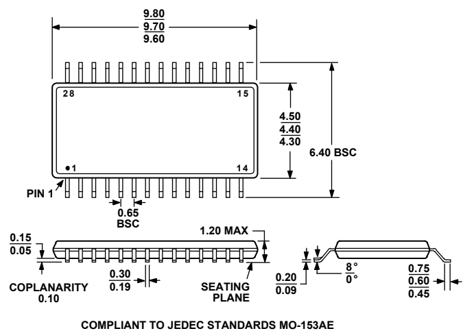
COMPLIANT TO JEDEC STANDARDS MO-153AE Figure 65. 28-Lead Thin Shrink Small Outline Package [TSSOP] (RU-28) Dimensions shown in millimeters
