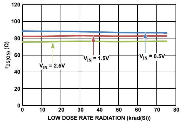
FIGURE 42. r_{DS(on)} ( V^+ = 3V ) - GROUNDING
