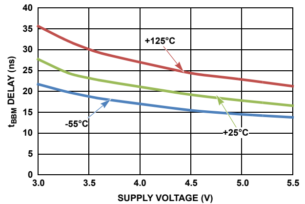
FIGURE 20. BREAK-BEFORE-MAKE DELAY
