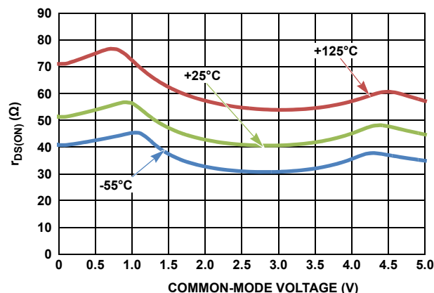
FIGURE 2. r_{DS(ON)} vs COMMON-MODE VOLTAGE ( V^+ = 5\text{V} )
