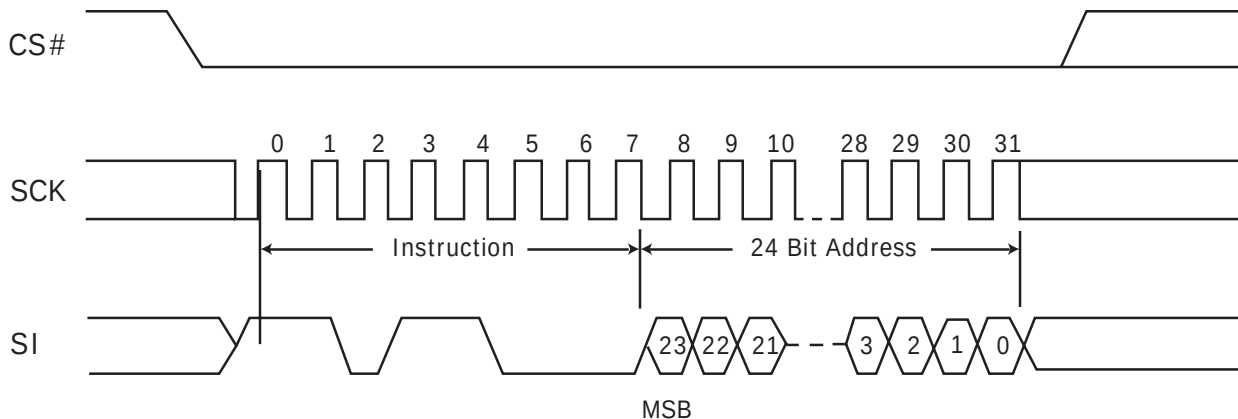
Figure I2. Sector Erase (SE) Instruction Sequence
