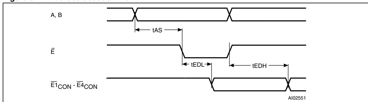
Figure 6. Address-decode time
