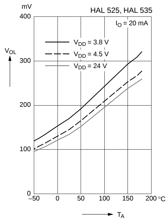
Fig. 3-10: Typical output low voltage versus ambient temperature
