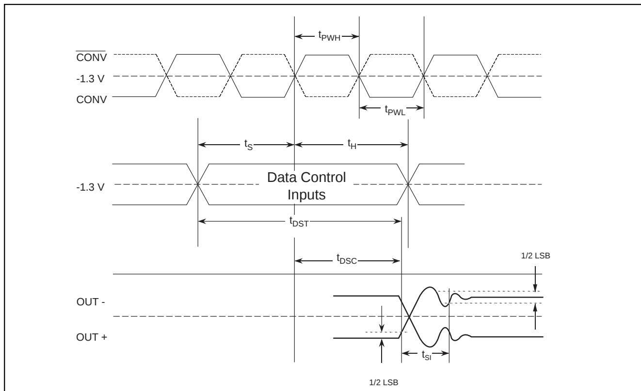
Figure 4. Timing Diagram
