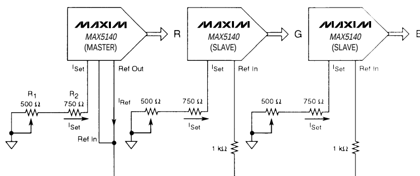
Figure 8. Typical RGB Graphics System
