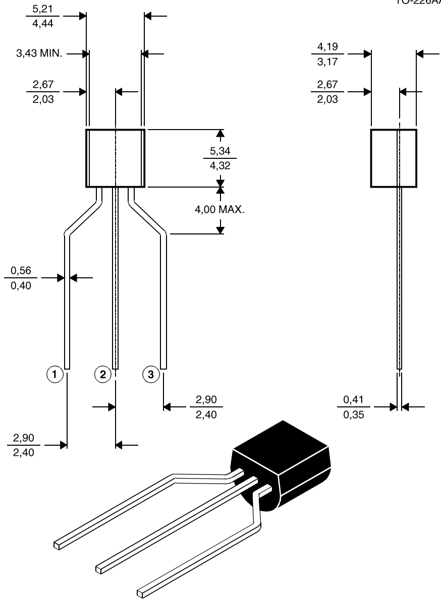
LP003 (TO-92) - Formed Leads Version
