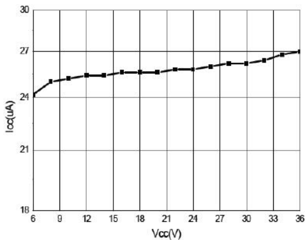
Figure 2. Drive Current Vs. Vcc Voltage
