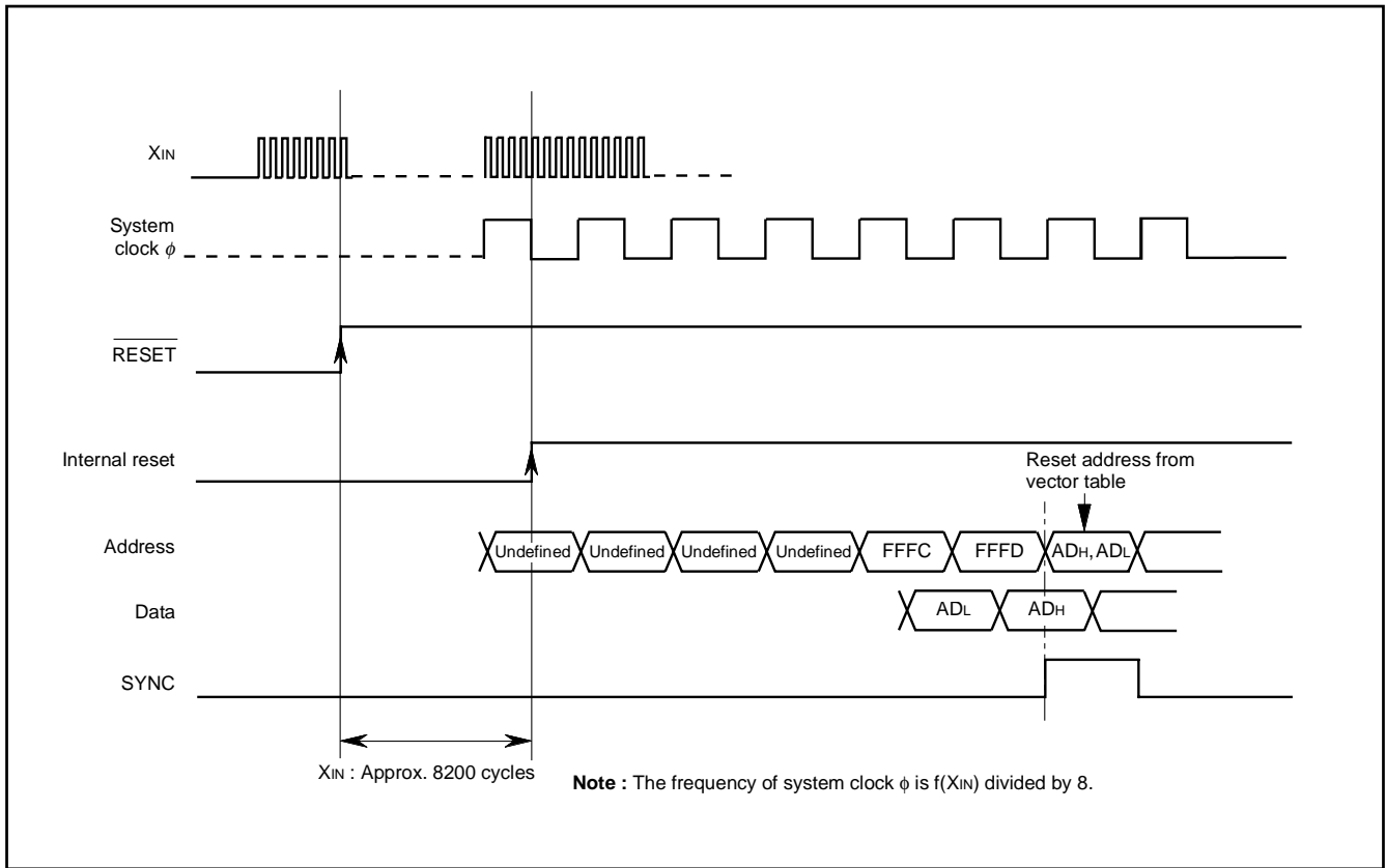
Fig. 57 Reset Sequence
