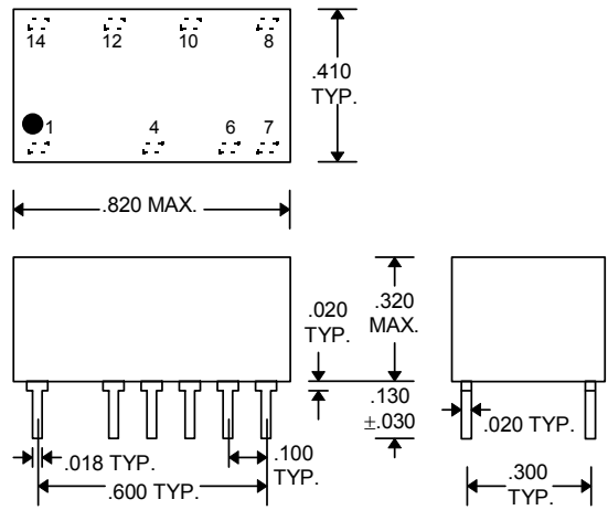
DDU66C-xxME7 (Military)
