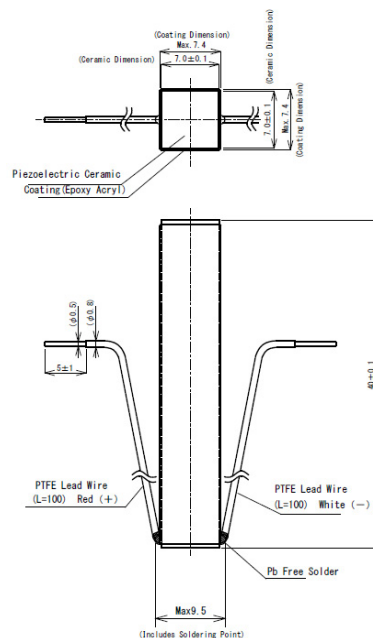
AE0707D44H40DF
