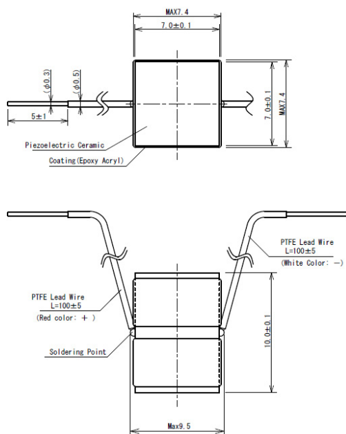
AE00707D08DF
