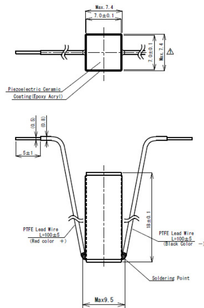
AE0707D18H18DF
