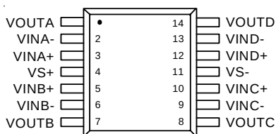
TSSOP-14 RT9139A
