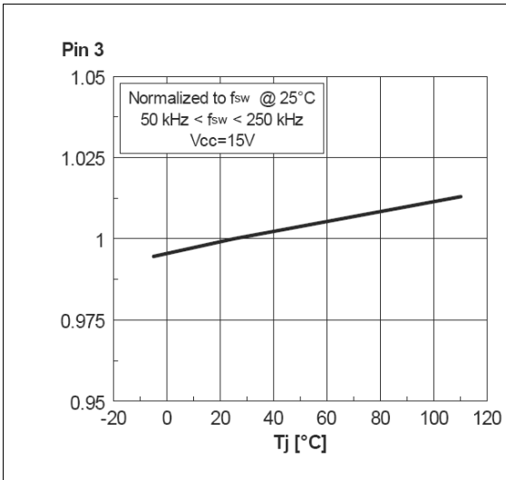
Figure 8. Oscillator frequency vs junction temperature
