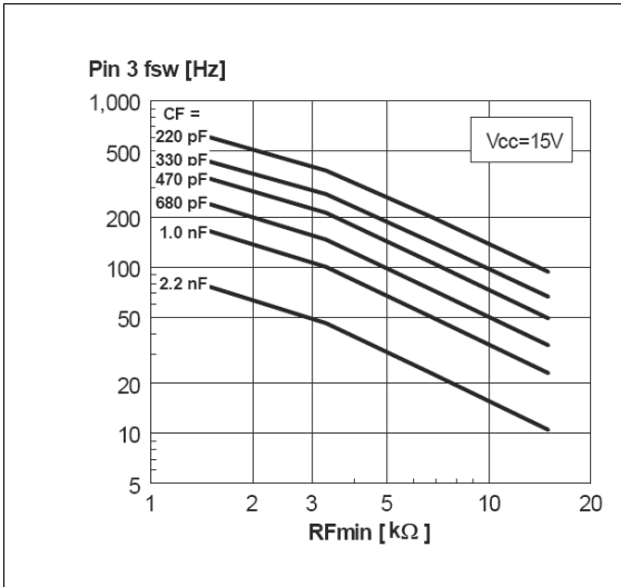
Figure 10. Oscillator frequency vs timing components
