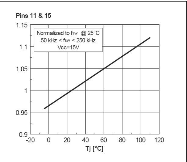
Figure 9. Dead-time vs junction temperature
