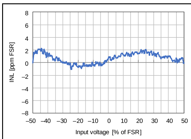
Figure 2.92 Input Voltage Dependence of Integral Non-Linearity ( AVCC0 = 5.0\text{ V} , T_a = 25^\circ\text{C} , Normal Mode, Gain = 2, OPCR.DSADLVM bit = 0, V_{REF} = 2.5\text{ V} )
