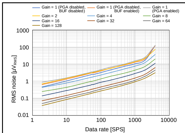
Figure 2.89 Data Rate Dependence of RMS Noise (AVCC0 = 5.0 V, T_a = 25^\circ\text{C} , Low Power Mode, V_{ID} = 0\text{V} , V_{REF} = 2.5\text{V} )
