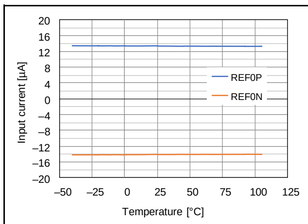
Figure 2.107 Temperature Dependence of External Reference Input Current ( AVCC0 = 5.0\text{ V} , Reference Buffer Disabled)
