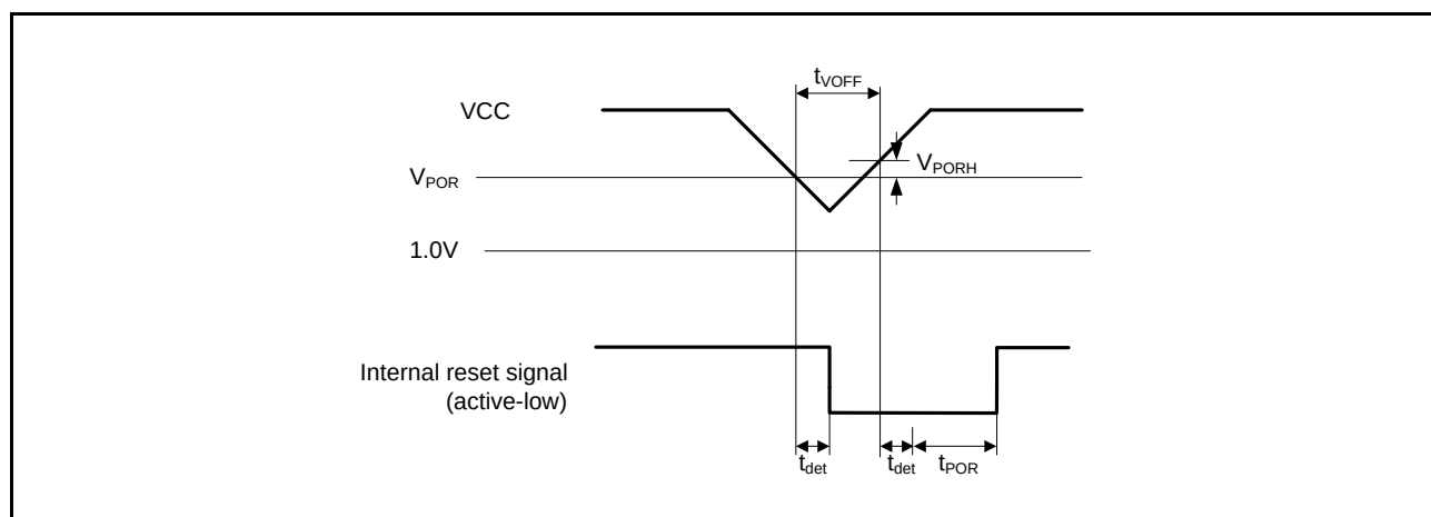
Figure 2.69 Voltage Detection Reset Timing
