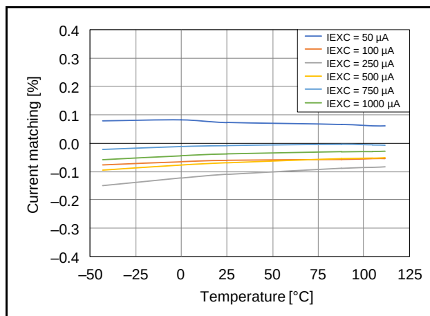
Figure 2.105 Temperature Dependence of Matching of Output Current of Excitation Current Source ( AVCC0 = 5.0\text{ V} )
