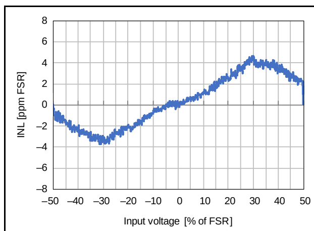
Figure 2.93 Input Voltage Dependence of Integral Non-Linearity ( AVCC0 = 5.0\text{ V} , T_a = 25^\circ\text{C} , Normal Mode, Gain = 1 (PGA disabled, BUF disabled), OPCR.DSADLVM bit = 0, V_{REF} = 2.5\text{ V} )
