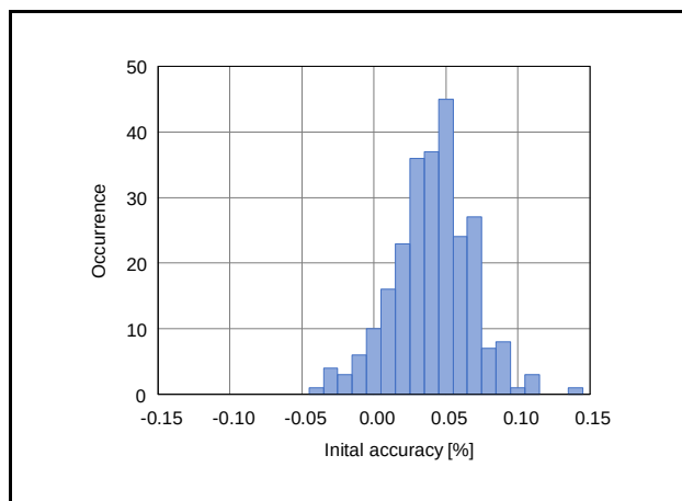
Figure 2.99 Initial Accuracy of Voltage Reference (AVCC0 = 5.0 V)
