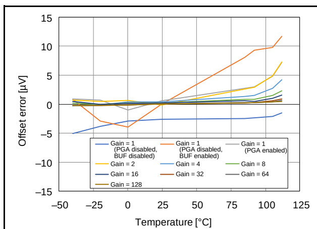
Figure 2.94 Temperature Dependence of Offset Error ( AVCC0 = 5.0\text{ V} , V_{ID} = 0\text{ V} , V_{REF} = 2.5\text{ V} )
