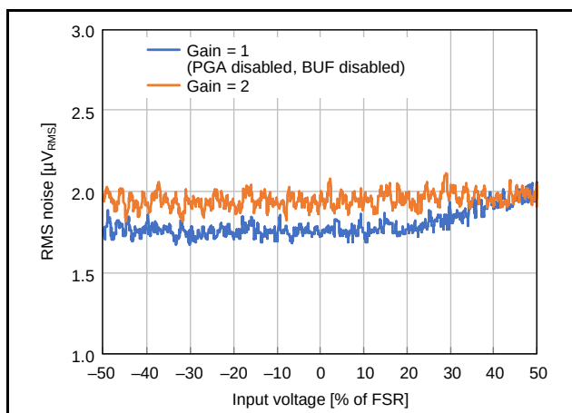
Figure 2.91 Input Voltage Dependence of RMS Noise (AVCC0 = 5.0 V, T_a = 25^\circ\text{C} , Normal Mode, f_{DR} = 122\text{ SPS} , V_{REF} = 2.5\text{V} )
