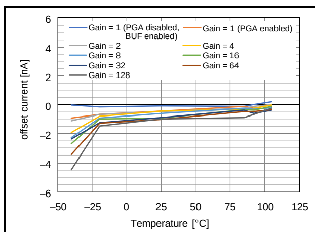
Figure 2.97 Temperature Dependence of Analog Input Offset Current ( AVCC0 = 5.0\text{ V} )
