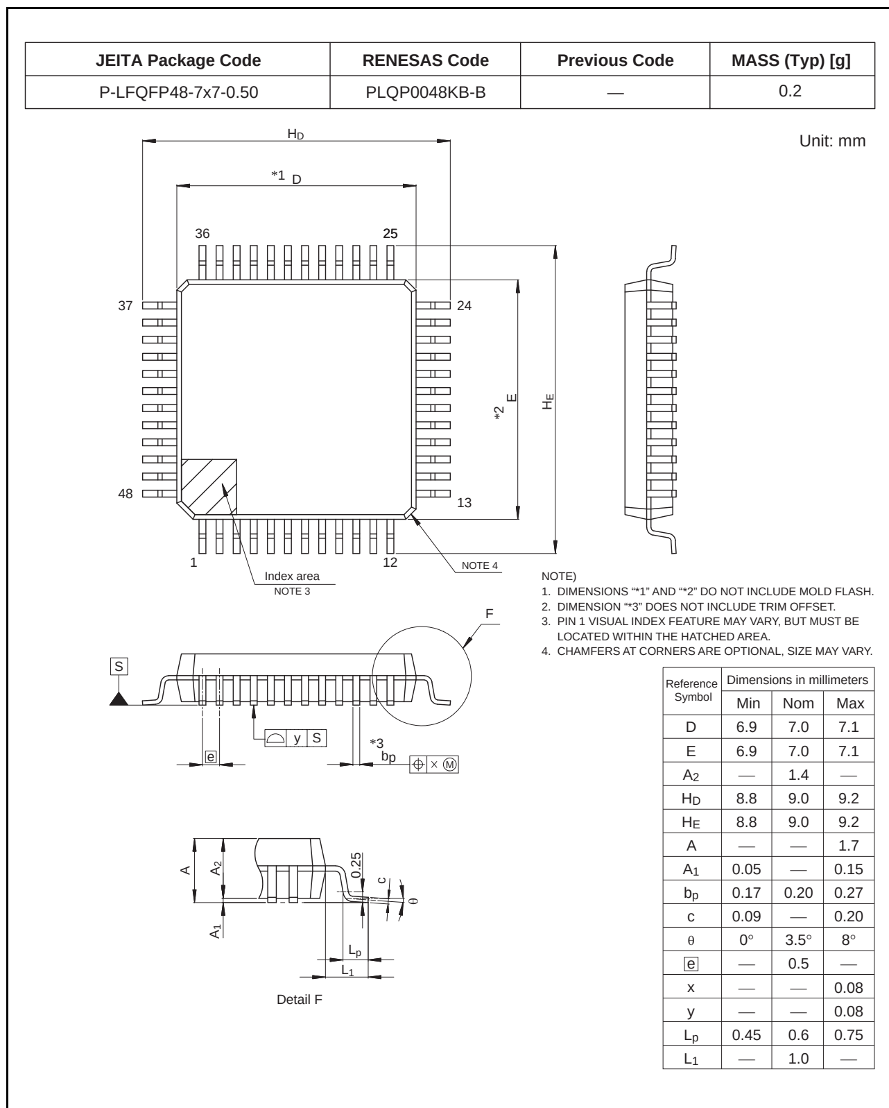
Figure A 48-Pin LFQFP (PLQP0048KB-B)
