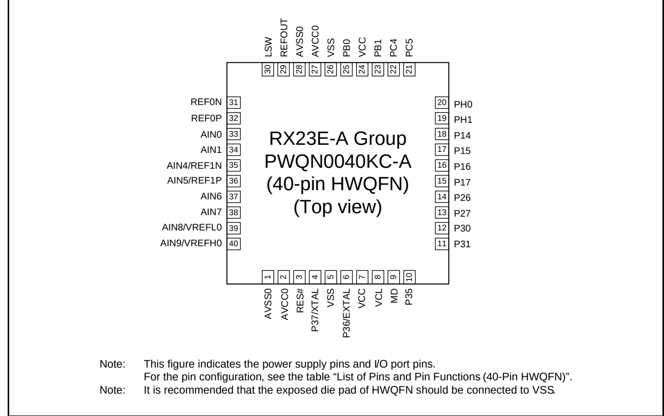
Figure 1.4 Pin Assignments of the 40-Pin HWQFN
