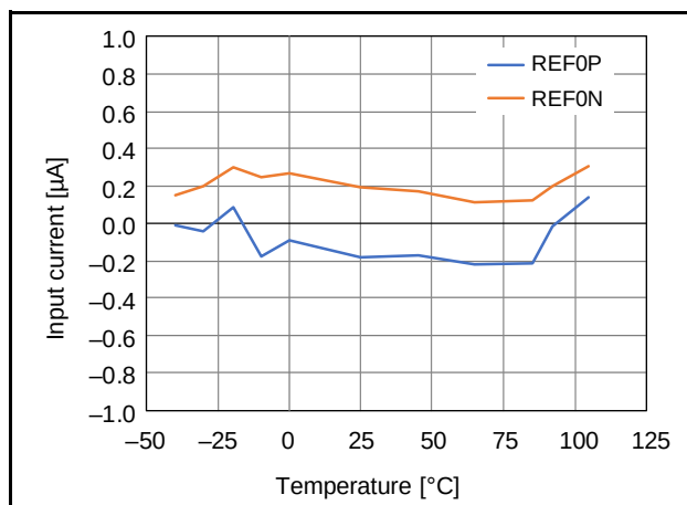
Figure 2.108 Temperature Dependence of External Reference Input Current ( AVCC0 = 5.0\text{ V} , Reference Buffer Enabled)
