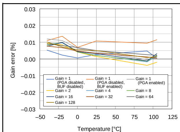
Figure 2.95 Temperature Dependence of Gain Error ( AVCC0 = 5.0\text{ V} , OPCR.DSADLVM bit = 0, V_{REF} = 2.5\text{ V} )
