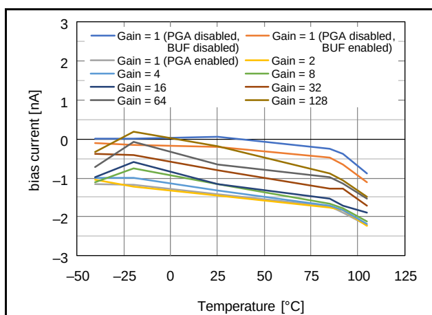
Figure 2.96 Temperature Dependence of Analog Input Bias Current ( AVCC0 = 5.0\text{ V} )
