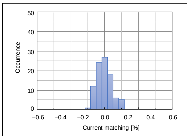
Figure 2.104 Matching of Output Current of Excitation Current Source ( AVCC0 = 5.0\text{ V} , T_a = 25^\circ\text{C} , I_{EXC} = 250\text{ }\mu\text{A} , 93 samples)
