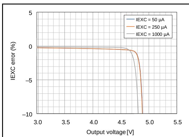
Figure 2.106 IEXC Accuracy vs Compliance Voltage ( AVCC0 = 5.0\text{ V} , T_a = 25^\circ\text{C} )
