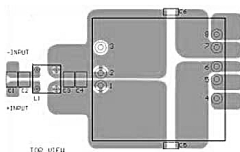
Recommended Layout with input Filter
