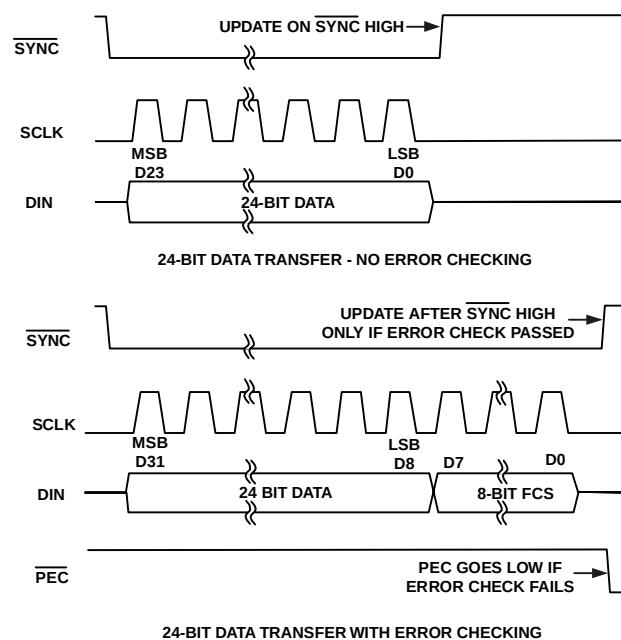
Figure 10. SPI Write With and Without Error Checking
