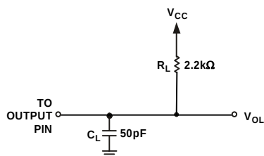
Figure 2. Load Circuit for \overline{BUSY} Timing
