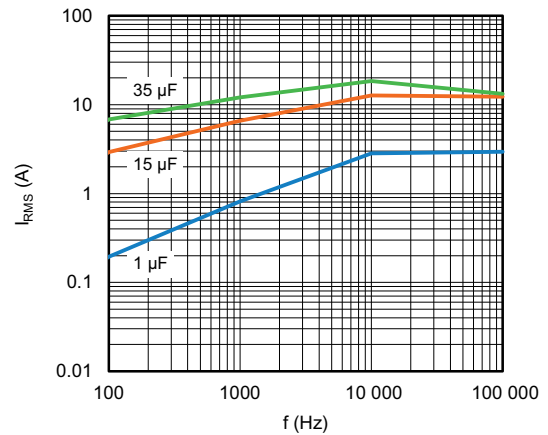
Maximum RMS current as function of frequency T_{amb} \leq 85\text{ }^{\circ}\text{C} ; U_r = 310\text{ V}_{AC}
