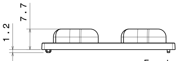
Front view Scale: 3:2
