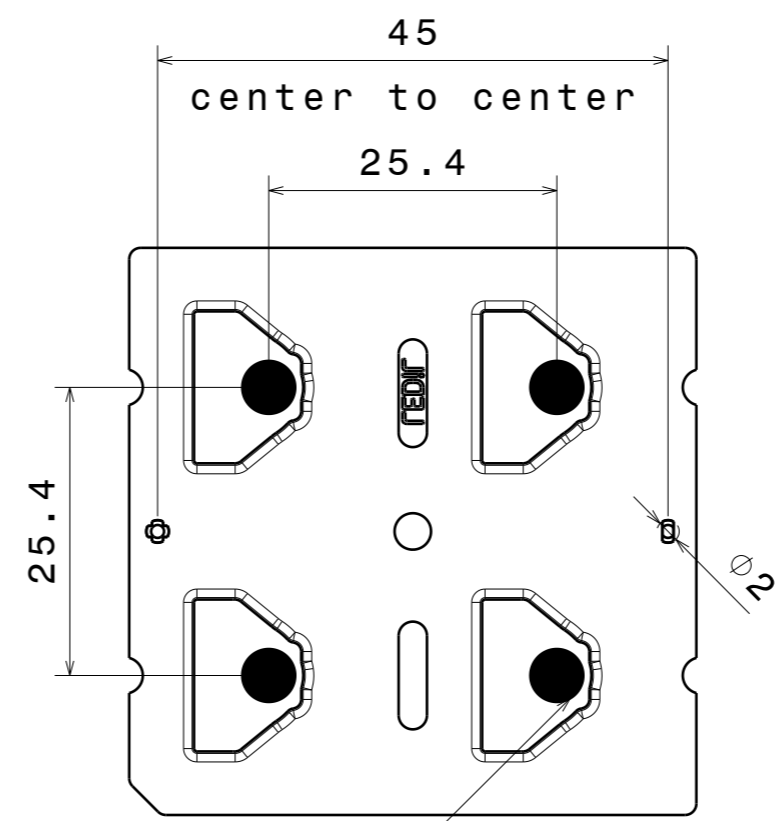
LED position Bottom view Scale: 3:2
