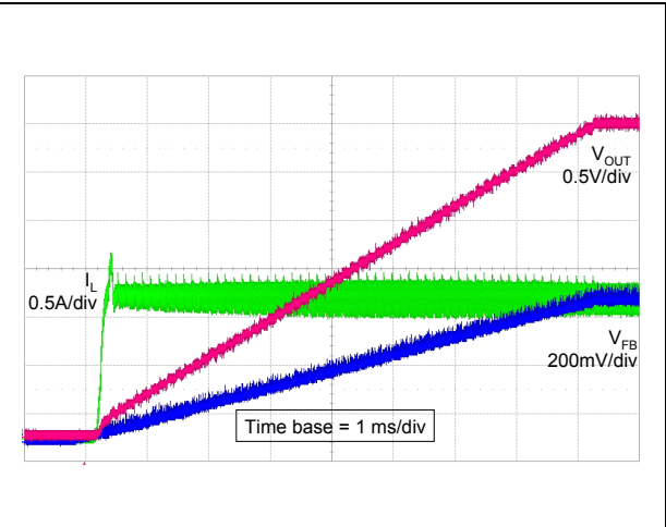
Figure 31. Soft-start
