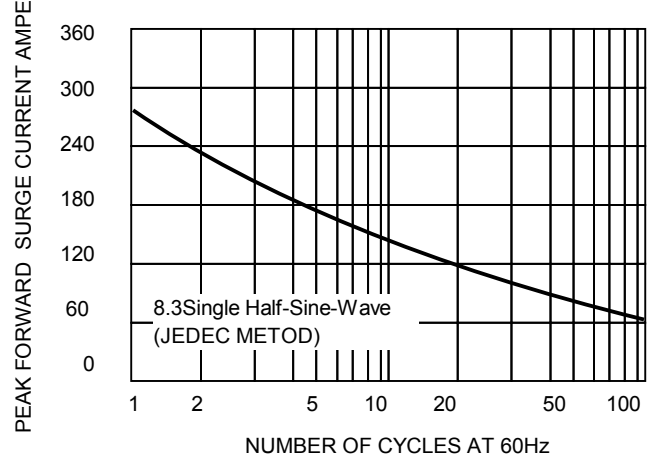
FIG.2-MAXIMUM NON-REPETITIVE SURGE
