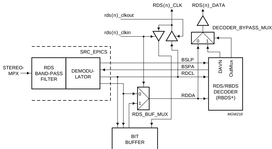
Fig.27 RDS/RBDS functional block diagram.
