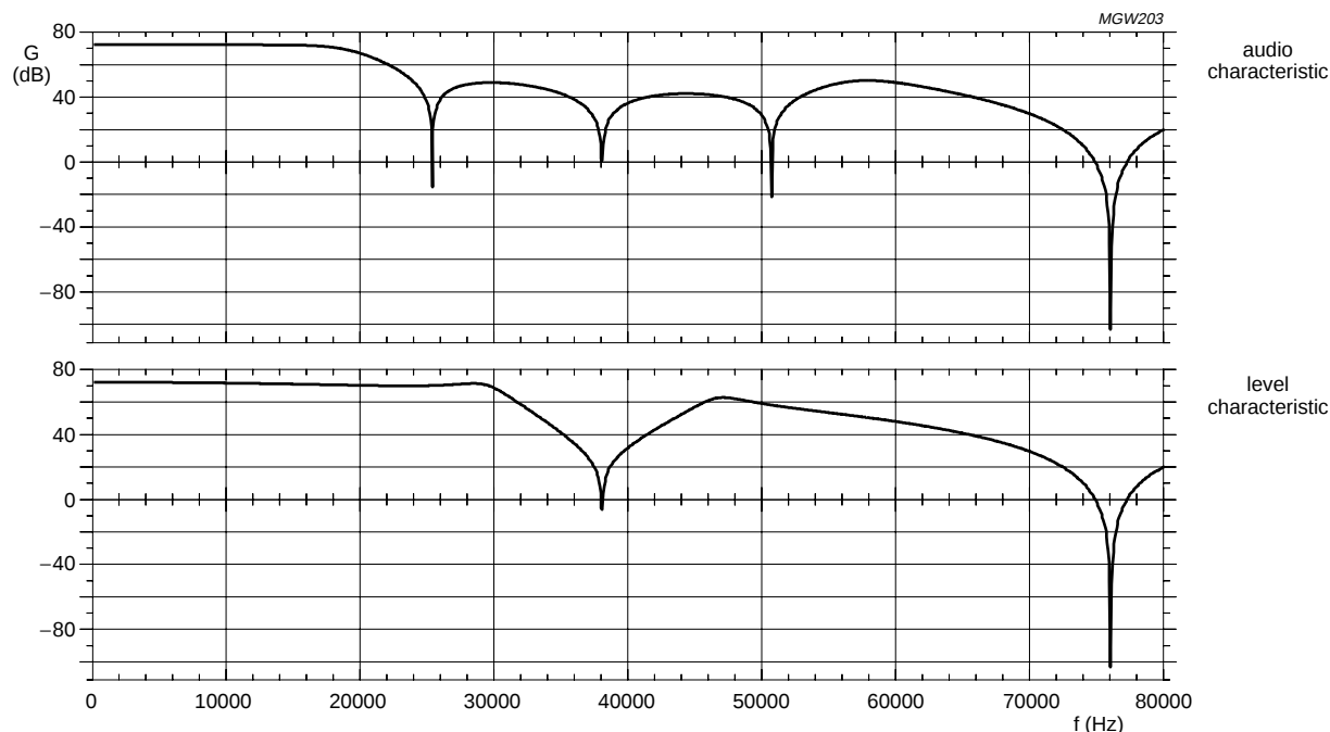
Fig.13 AUX decimation path transfer characteristics.
