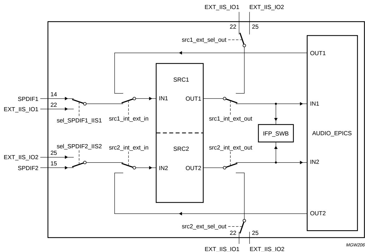
Fig.16 SRC audio signal flows.
