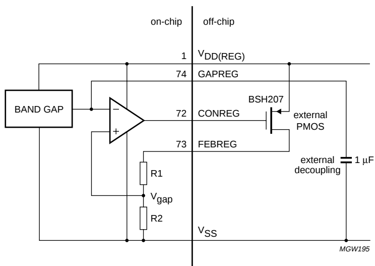
Fig.5 Voltage regulator schematic diagram.
