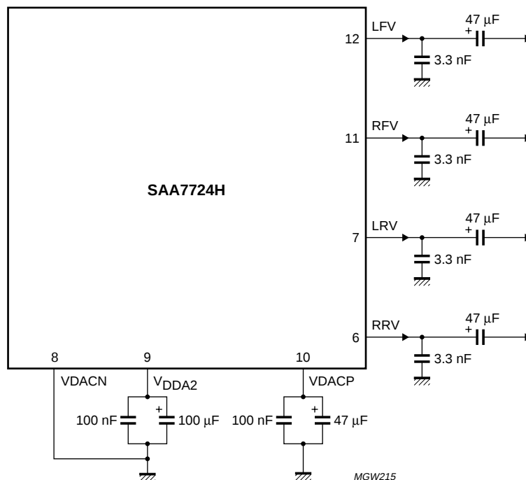
Fig.25 DAC outputs application diagram.
