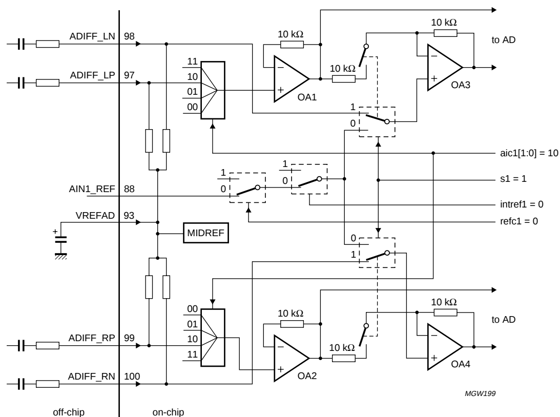
Fig.9 Example of the use of differential analog input ADIFF_L and ADIFF_R.
